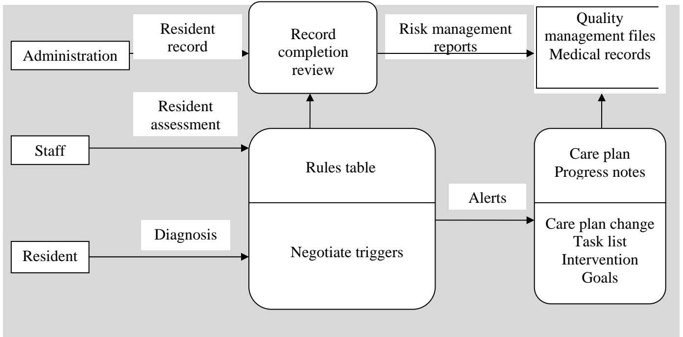
Data Flow Diagram of Nursing Home Clinical Information System with Decision Support
